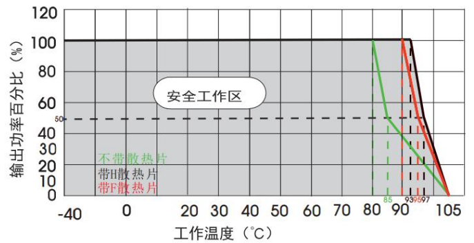
WLD10-H1D24/28/48/54(F/H)温度降额曲线 (Vin=110V, 无风)
