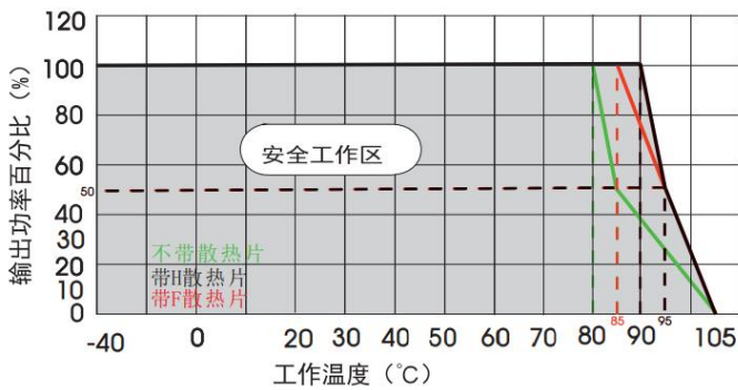
WLD10-H1D03/05/12/15(F/H)温度降额曲线 (Vin=110V, 无风)
