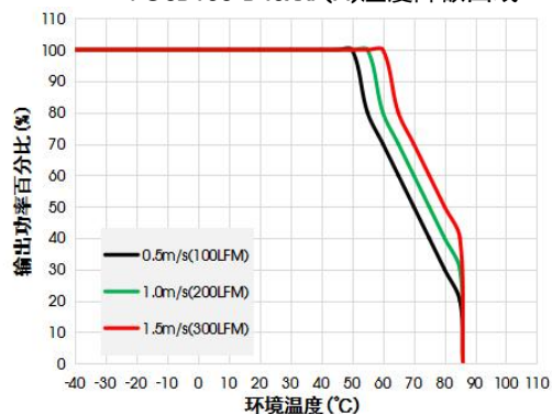
VOSB100-B48xxF(N)温度降额曲线
