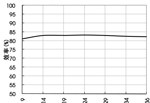
UP6-H2405 效率Vs输入电压 (满载)
