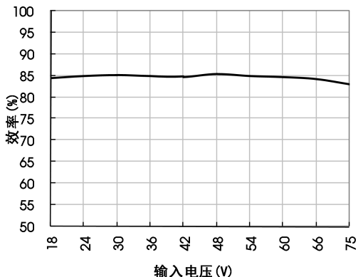
UP6-H4815 效率Vs输入电压 (满载)
