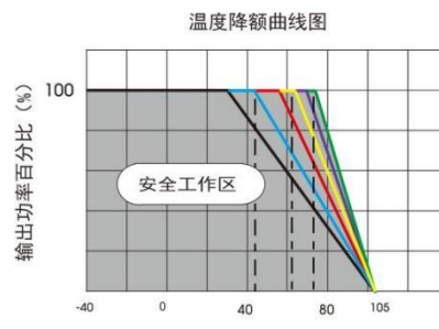
UHB150-F1D48H 温度降额曲线(Vin=110V)
