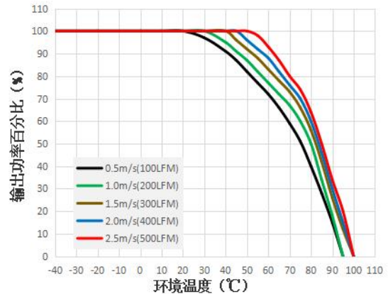
UFB400-F1D05H 温度降额曲线图
