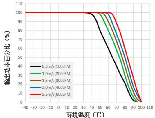
UFB400-F1D24H 温度降额曲线图
