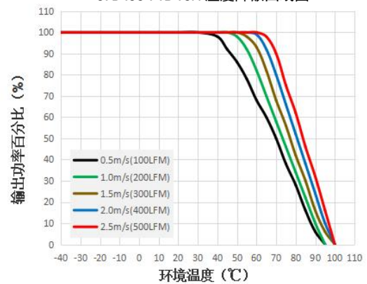
UFB400-F1D24H 温度降额曲线图
