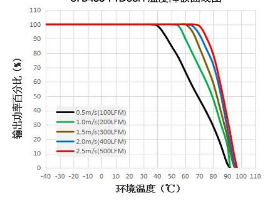
UFB400-F1D48H 温度降额曲线图
