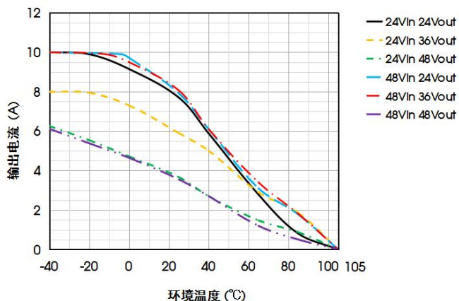
KEB10-UB4836(-RS)温度降额曲线 (20LFM)
