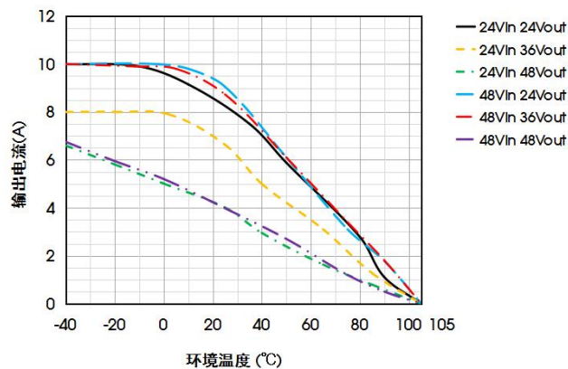
KEB10-UB4836F(-RS)温度降额曲线 (20LFM)
