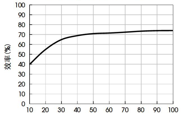
输出电流百分比 (%) (DXT1-IB1205)
