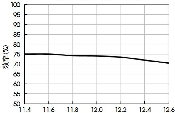
输入电压 (V) (DXT1-IB1205)
