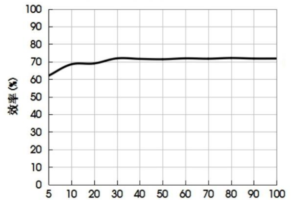
输出电流百分比 (%) (DXT1-IB0503)
