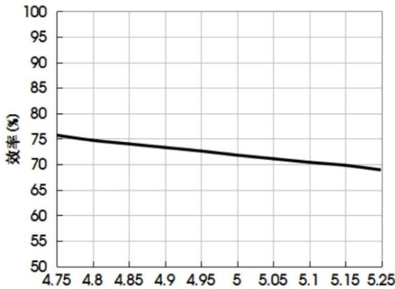
输入电压 (V) (DXT1-IB0503)
