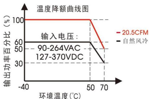
24/36V-C(满载 350W 带 20.5CFM 风扇)
