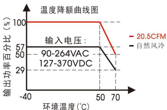
24/36V-C(满载 350W 带 20.5CFM 风扇)
