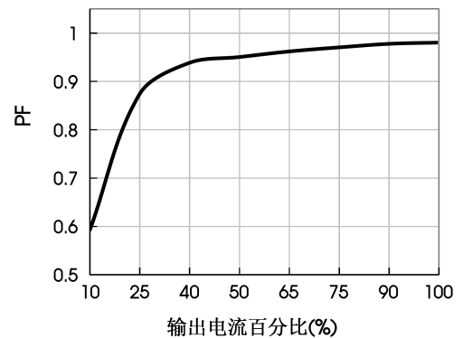
PF Vs 输出负载 (Vin=230VAC)
